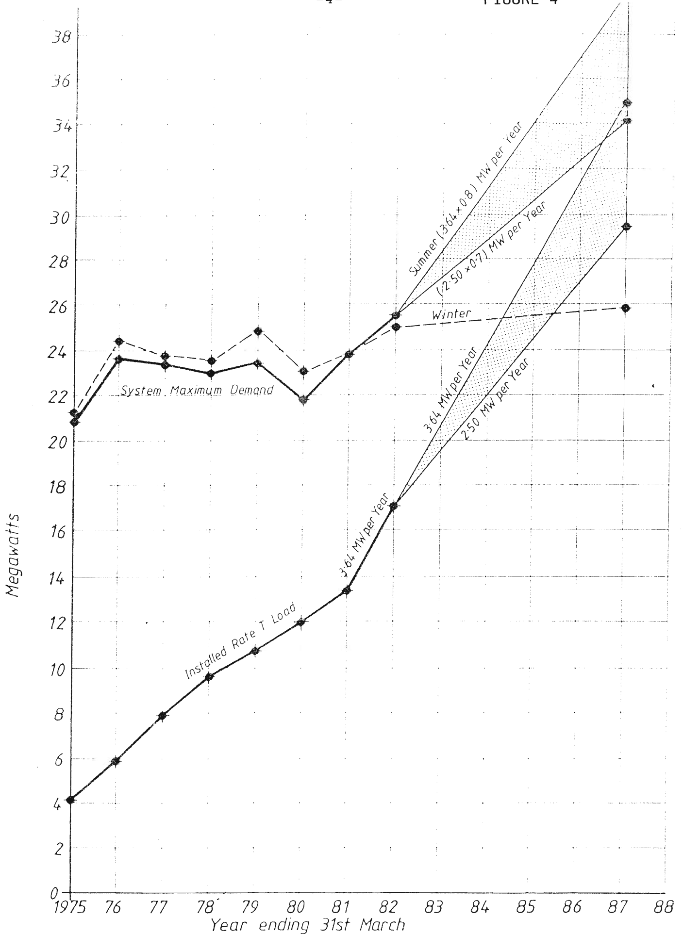
Ashburton Electric Power Board SUMMER AND WINTER SYSTEM MAXIMUM DEMANDS AND INSTALLED IRRIGATION LOAD Recorded 1975-82 and projected to 1987
