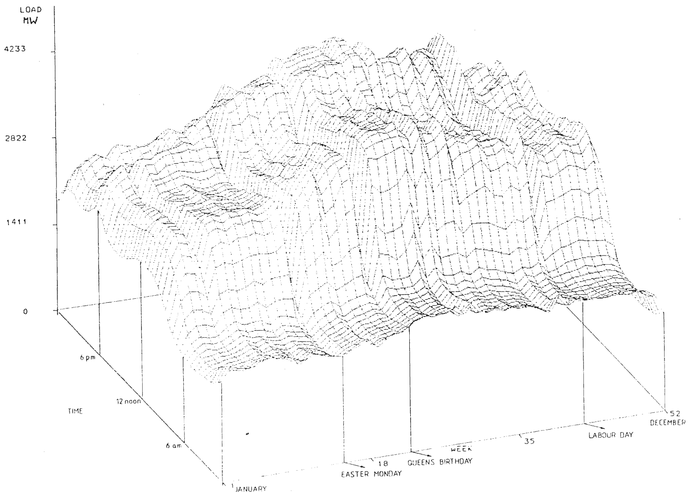
LOAD ON MONDAYS IN 1982
