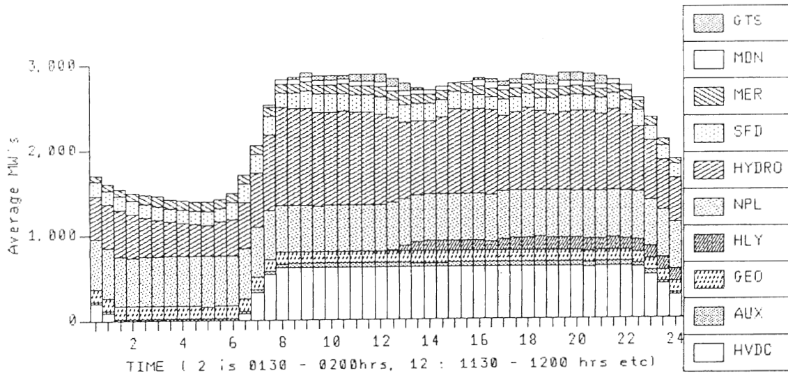
NORTH ISLAND half-hourly generation for 8 JULY 1982.
