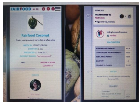
Figure 7: FairFood Blockchain
